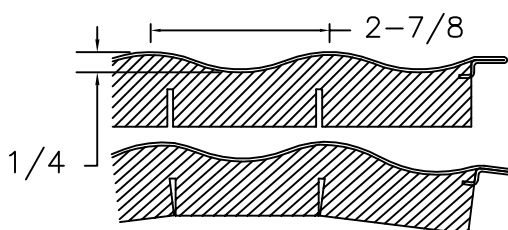
TANKPANEL DETAIL
